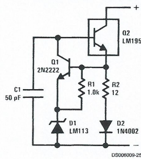
Two Terminal 100 mA Current Regulator
