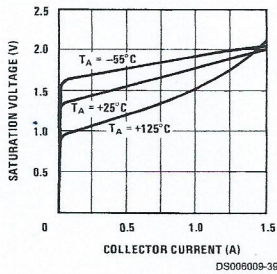
Saturation Voltage
