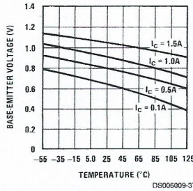
Base Emitter Voltage
