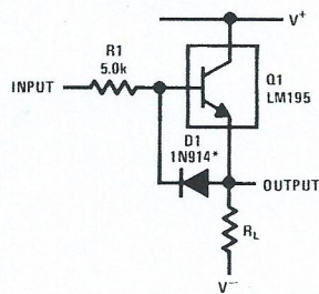
Fast Follower
