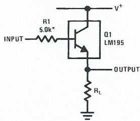
Emitter Follower
