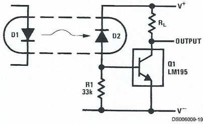
Fast Optically Isolated Switch
