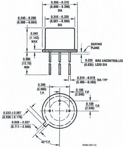
TO-5 Metal Can Package Order Number LM195H/883 NS Package Number H03B
