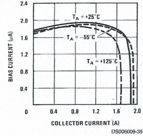
Bias Current
