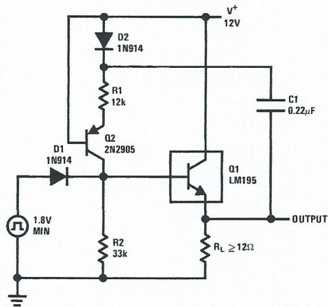
Power One-Shot
