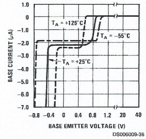
Base Current
