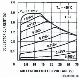
Collector Characteristics
