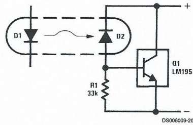
Optically Isolated Power Transistor
