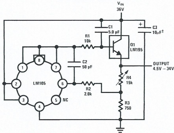
1.0 Amp Positive Voltage Regulator
