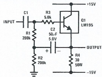
High Input Impedance AC Emitter Follower
