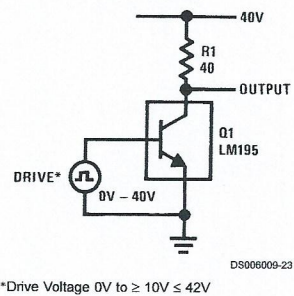
40V Switch
