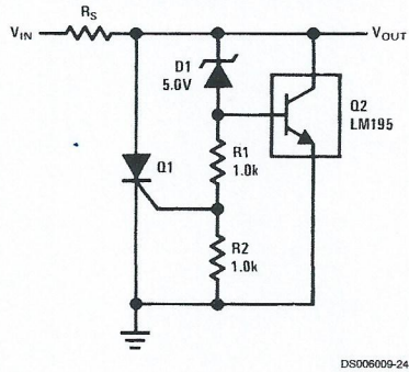
6.0V Shunt Regulator with Crowbar
