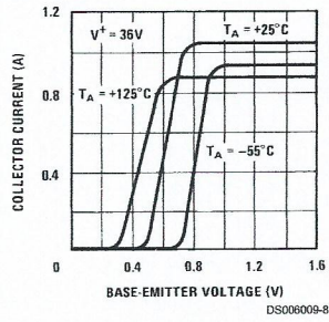
36V Transfer Function
