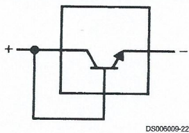
Two Terminal Current Limiter
