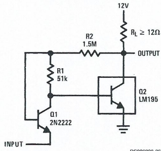
Low Level Power Switch
