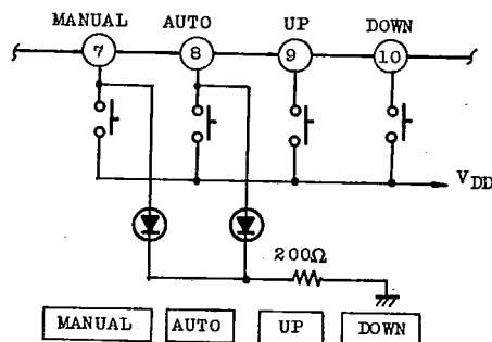
When MANUAL/AUTO Lock key is used.
