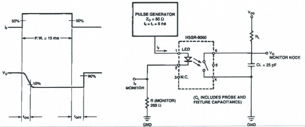
Figure 8. Switching Test Circuit for t_{ON} , t_{OFF} .
