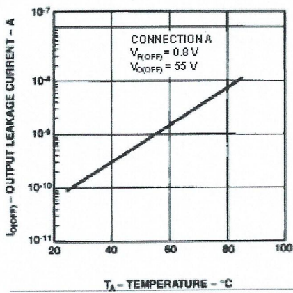
Figure 13. Typical Output Leakage vs. Temperature.
