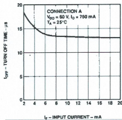
Figure 12. Typical Turn Off Time vs. Input Current.
