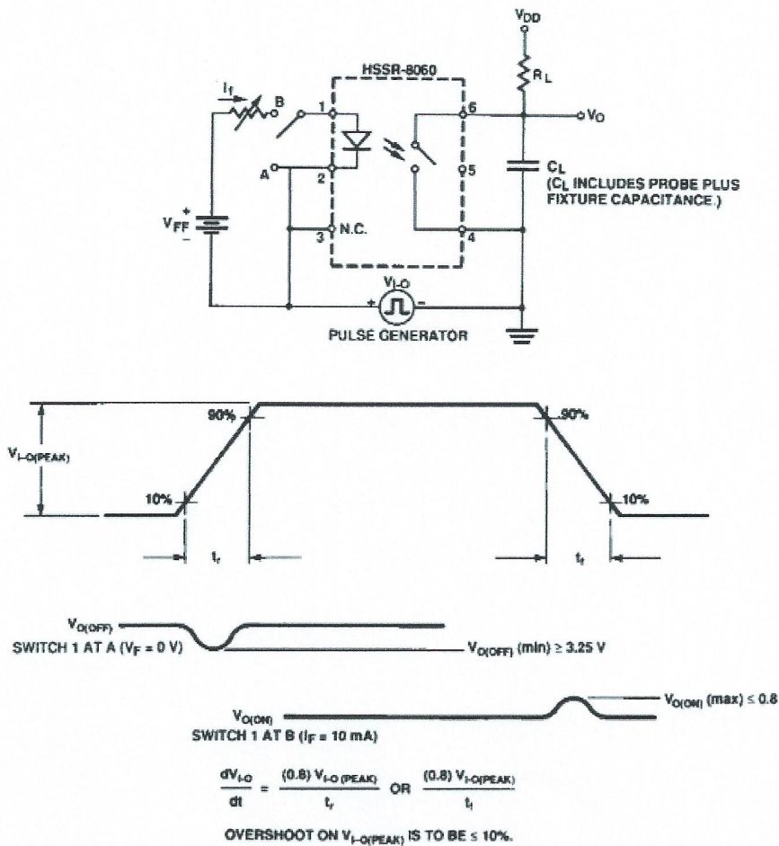
Figure 17. Input-Output Transient Rejection Test Circuit.
