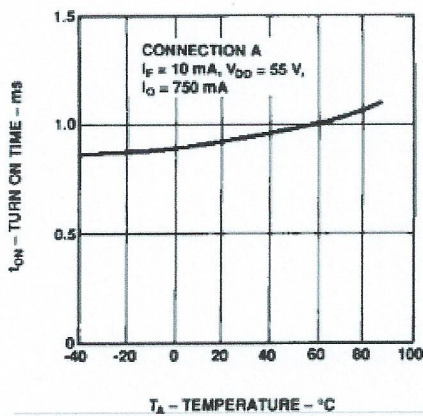
Figure 9. Typical Turn On Time vs. Temperature.
