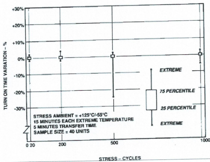
Figure 21. Turn On Time Variation with Temperature Cycling.
